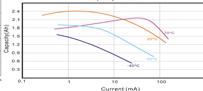
Capacity vs. Current
