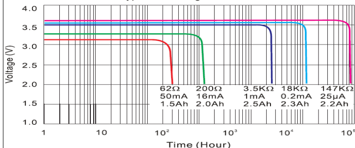
Typical Discharge Profile At 25°C
