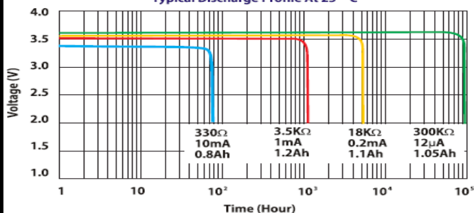
Typical Discharge Profile At 25° C
