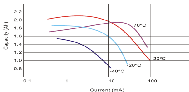
Capacity vs Current
