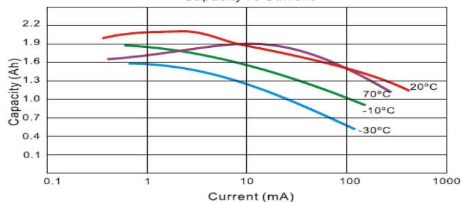
Capacity vs Current
