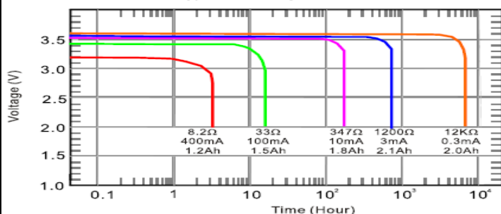
Typical Discharge Profile At 25°C
